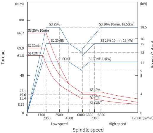
Mitsubishi Built-in Spindle (12000rpm)
