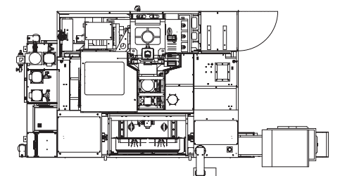
Diversified options for external chip conveyor
