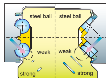
Contact between ball slideway and roller slideway.
